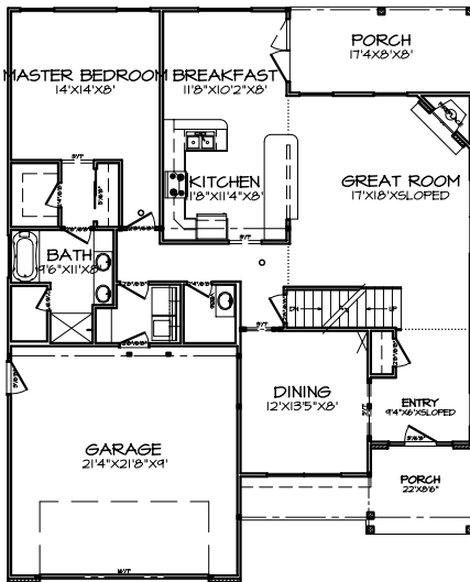
FIRST FLOOR PLAN A-4
